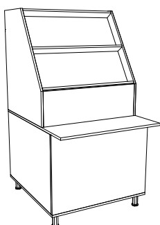
горка 2000x800x1000
